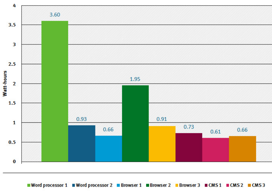
Figure 1: Comparison of energy consumption of the local device (SUT(Client)) during the execution of the standard usage scenario
